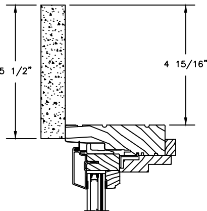
HEAD JAMB WITH 5 1/2" FLAT CASING
