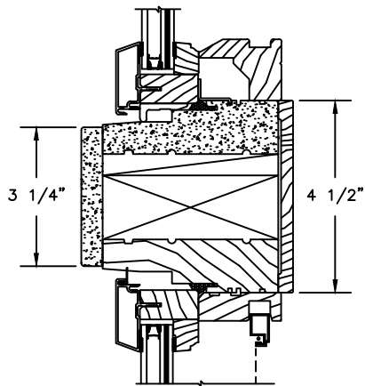
2" STRUCTURAL MULLION BY OTHERS
