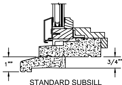
STANDARD SUBSILL
