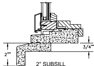
2" SUBSILL
