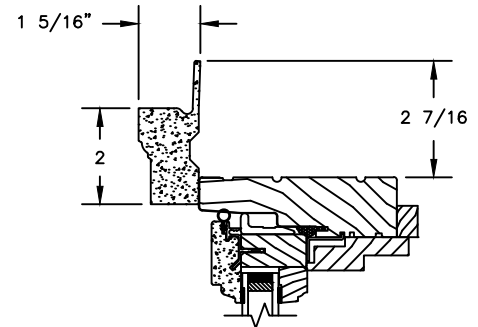
HEAD JAMB WITH 180 FLANGED BRICKMOULD
