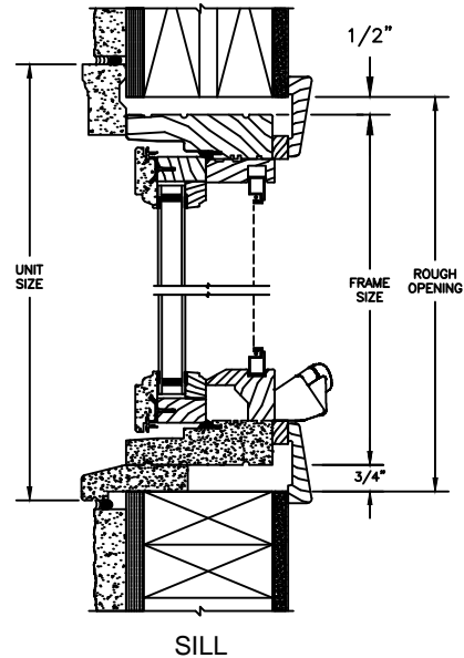
2 X 4 FRAME WITH STUCCO
