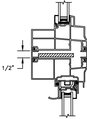
HORIZONTAL 1/2" MULLION RADIUS/OPERATOR
