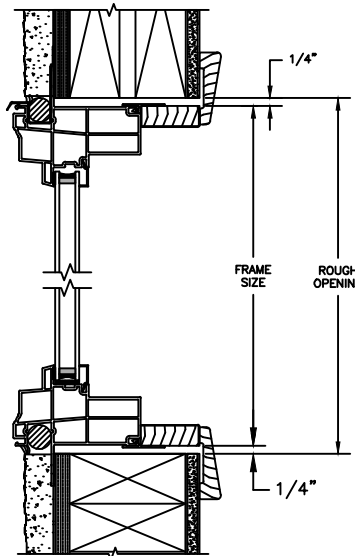
HEAD JAMB & SILL 2 X 4 FRAME WITH STUCCO
