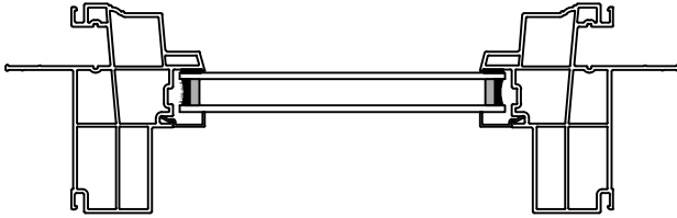
INSULATING GLASS
