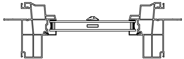
7/8" PUTTY WDL (EXTERIOR ONLY) WITH 13/16" FLAT INNERGRILLE
