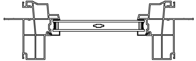
3/4" PROFILED INNERGRILLE
