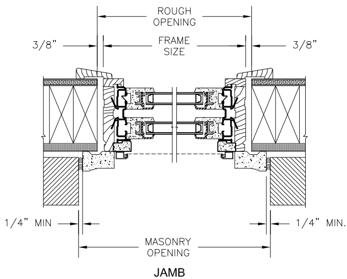
JAMB 2 X 4 FRAME WITH BRICK VENEER
