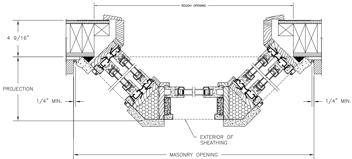
45 DEGREE BAY
