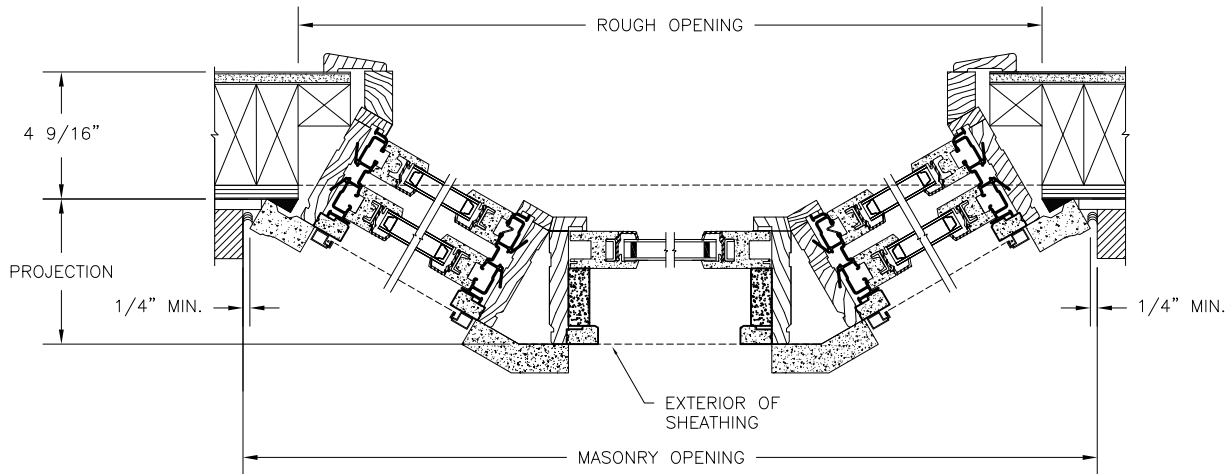
30 DEGREE BAY
