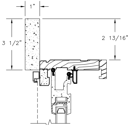
HEAD JAMB WITH 3 1/2" FLAT CASING
