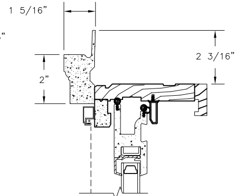
HEAD JAMB WITH 180 FLANGED BRICKMOULD
