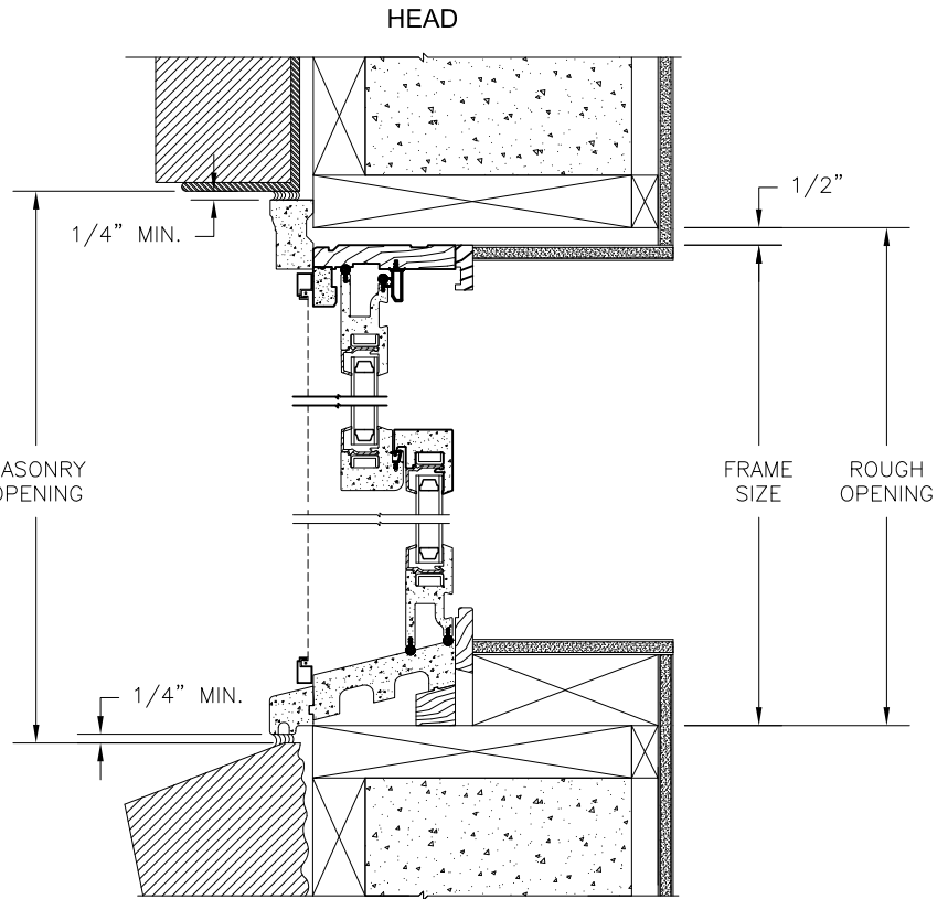
SILL 8" CONCRETE BLOCK WALL WITH BRICK VENEER
