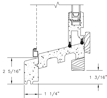
BULLNOSE SILLNOSE
