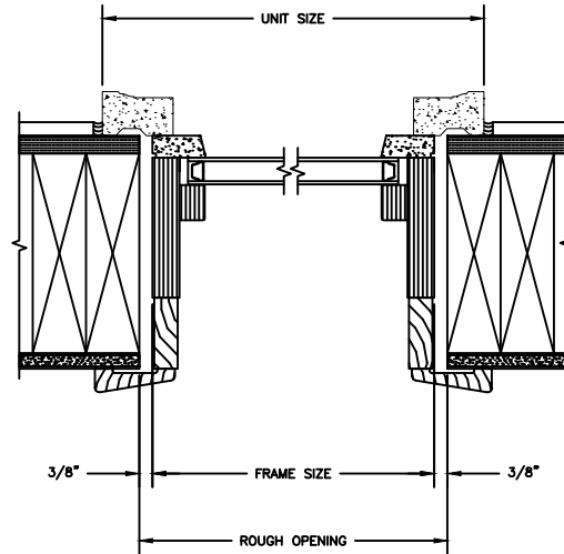
JAMBS 2 X 6 FRAME WITH SIDING
