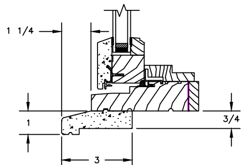
IN-SASH SILL WITH STANDARD SUBSILL
