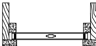
1" PROFILED INNERGRILLE
