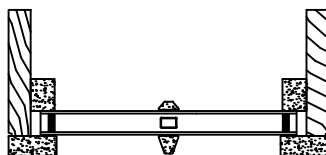
5/8" PUTTY (TALL) GLAZE WITH INNERBAR
