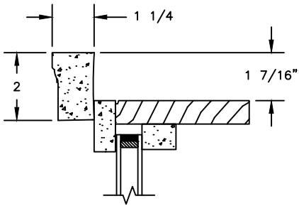
HEAD JAMB WITH STANDARD 180 BRICKMOULD
