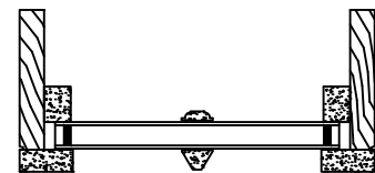
7/8" PUTTY (TALL) GLAZE WITHOUT INNERBAR
