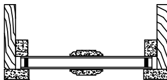
2" SIMULATED CHECK RAIL WITHOUT INNERBAR
