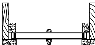
5/8" PUTTY (TALL) GLAZE WITHOUT INNERBAR
