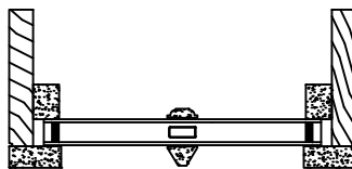
7/8" PUTTY (TALL) GLAZE WITH INNERBAR
