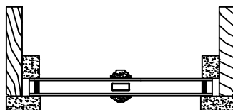
7/8" PUTTY (SHORT) GLAZE WITH INNER BAR
