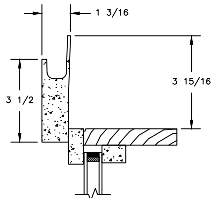
HEAD JAMB WITH 3 1/2" FLAT CASING WITH J-CHANNEL
