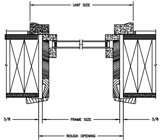
JAMBS 2 X 6 FRAME WITH SIDING
