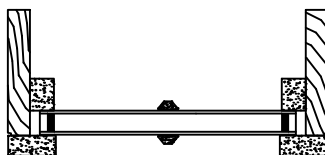
5/8" PUTTY (SHORT) GLAZE WITHOUT INNER BAR
