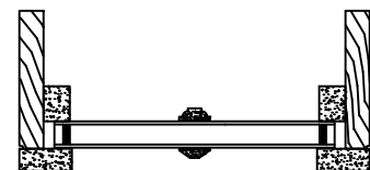
7/8" PUTTY (SHORT) GLAZE WITHOUT INNER BAR
