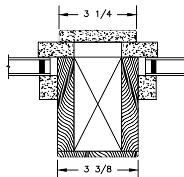
VERTICAL MULLION OPERATOR WITH 2" SPREAD MULL
