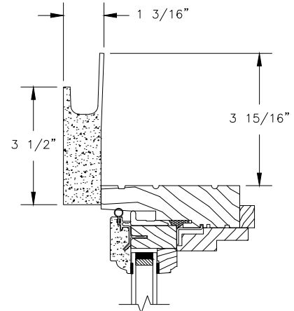
HEAD JAMB WITH 3 1/2" FLAT CASING WITH J-CHANNEL
