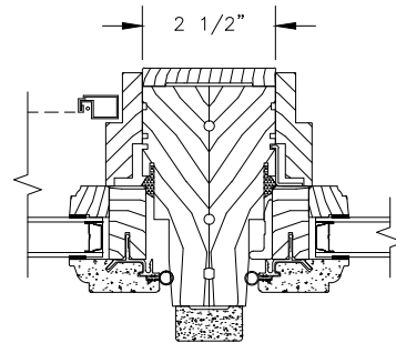
VERTICAL MULLION OPERATOR/PICTURE
