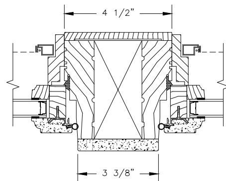
VERTICAL MULLION WITH 2" SPREAD MULL OPERATOR/OPERATOR
