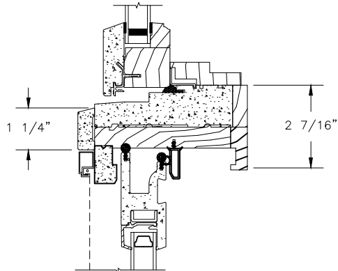
HORIZONTAL MULLION TRANSOM/OPERATOR
