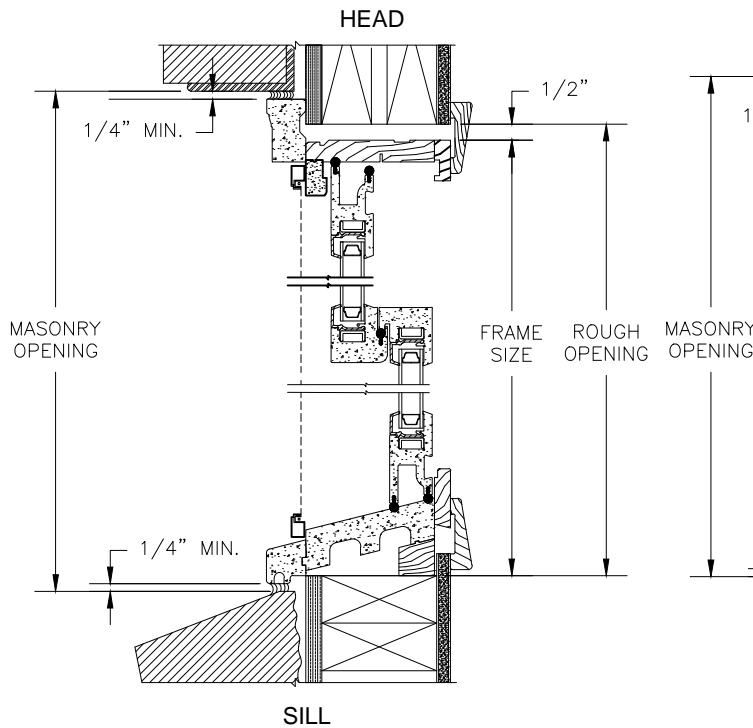
2 X 4 FRAME WITH BRICK VENEER
