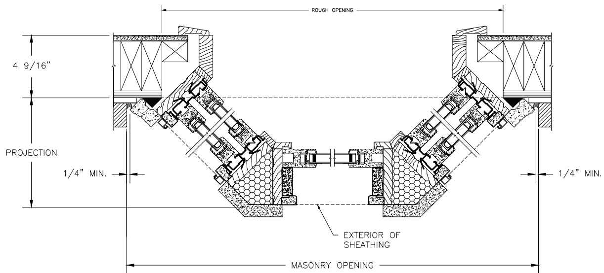
45 DEGREE BAY
