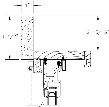
HEAD JAMB WITH 3 1/2" FLAT CASING
