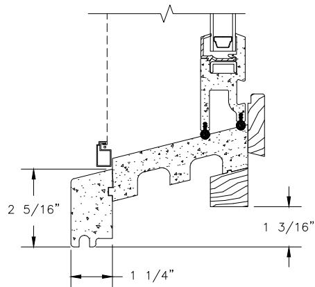
BULLNOSE SILLNOSE
