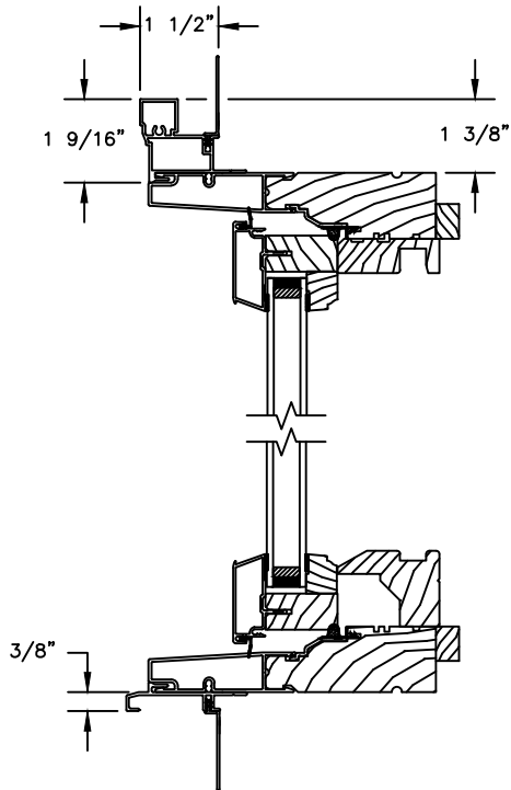
HEAD JAMB & SILL WITH CLAD BRICKMOULD CASING
