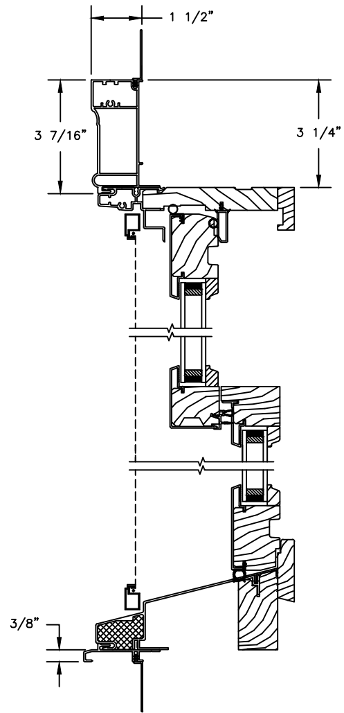
HEAD JAMB & SILL WITH CLAD WILLIAMSBURG CASING
