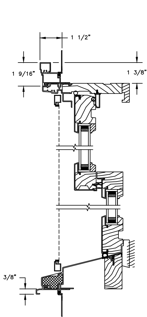
HEAD JAMB & SILL WITH CLAD BRICKMOULD CASING
