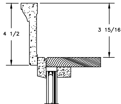
HEAD JAMB WITH 4 1/2" BACKBAND
