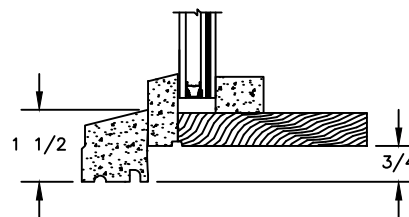
SILL WITH STANDARD SUBSILL
