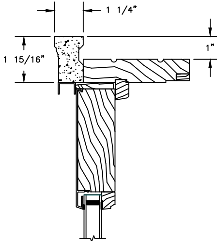
HEAD JAMB WITH STANDARD 180 BRICKMOULD
