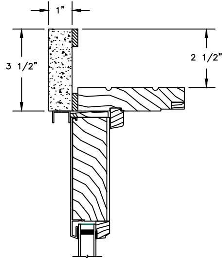
HEAD JAMB WITH 3 1/2" FLAT CASING
