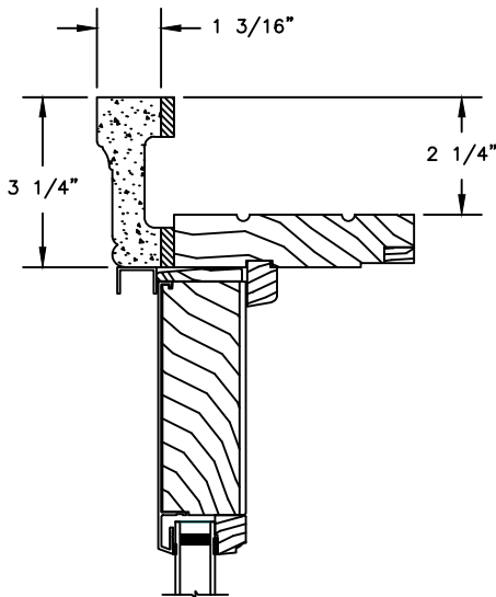
HEAD JAMB WITH WILLIAMSBURG BRICKMOULD
