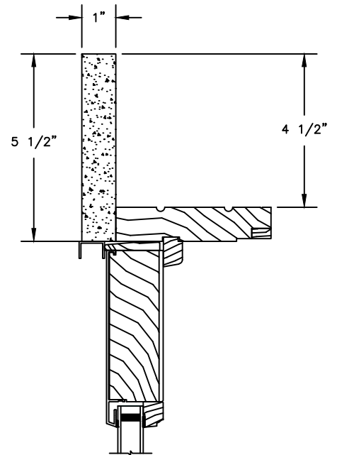
HEAD JAMB WITH 5 1/2" FLAT CASING
