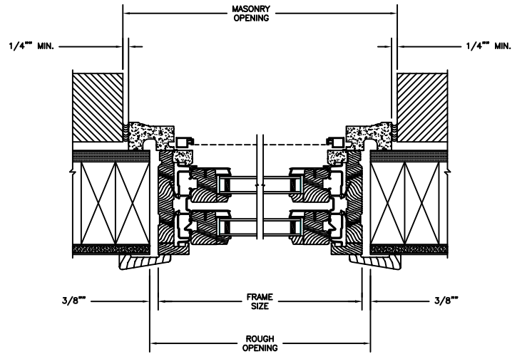
JAMB 2 X 4 FRAME WITH BRICK VENEER
