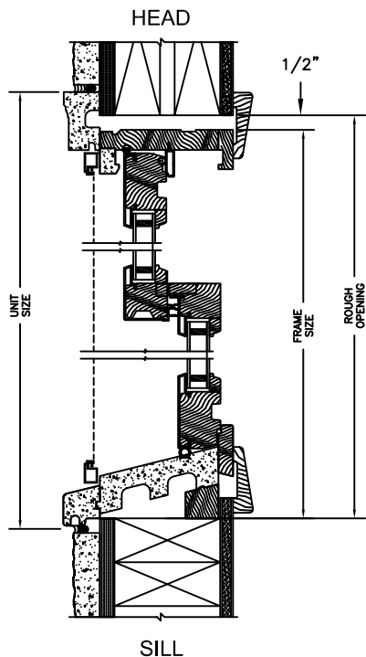
2 X 4 FRAME WITH STUCCO
